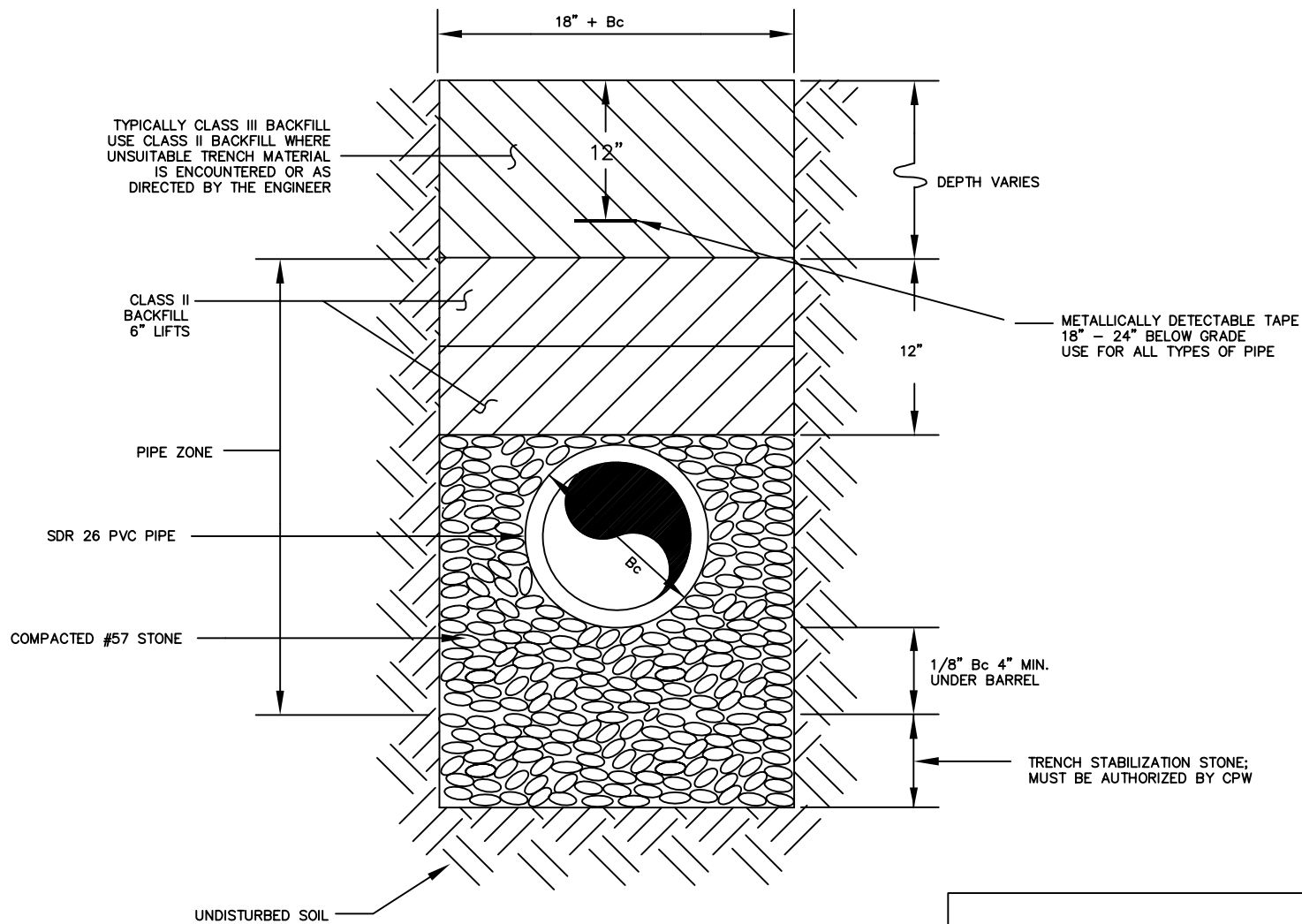
MINIMUM BEDDING FOR GRAVITY SEWER LINE
