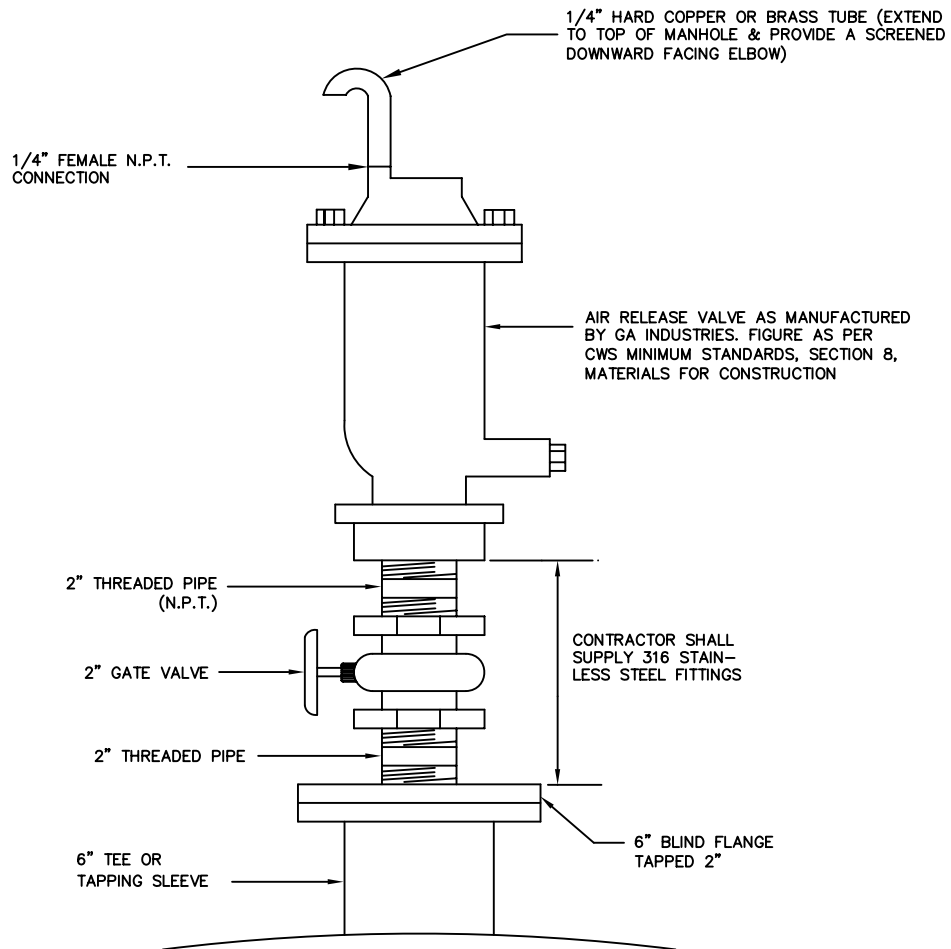
AIR RELEASE VALVE FOR WATER SYSTEM
